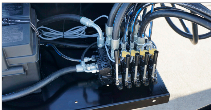
Hydraulic S-Drive
