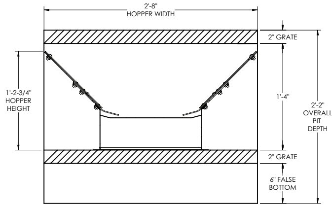
PIT DIMENSIONS
